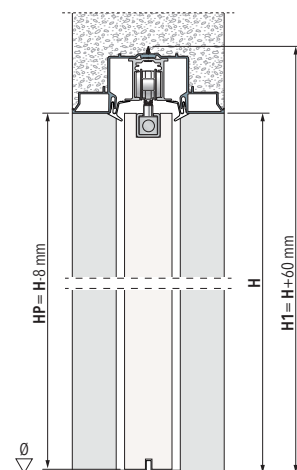
ECLISSE Syntesis Line
